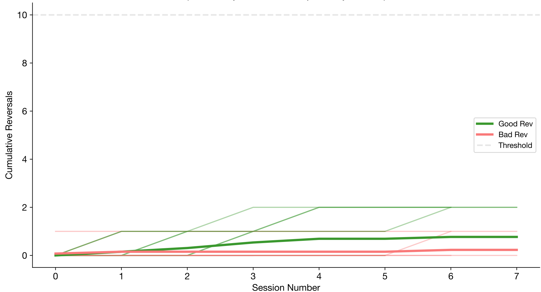
Cumulative Good and Bad Reversals Over Time (n=13 subjects; sessions per subject=1–8)
